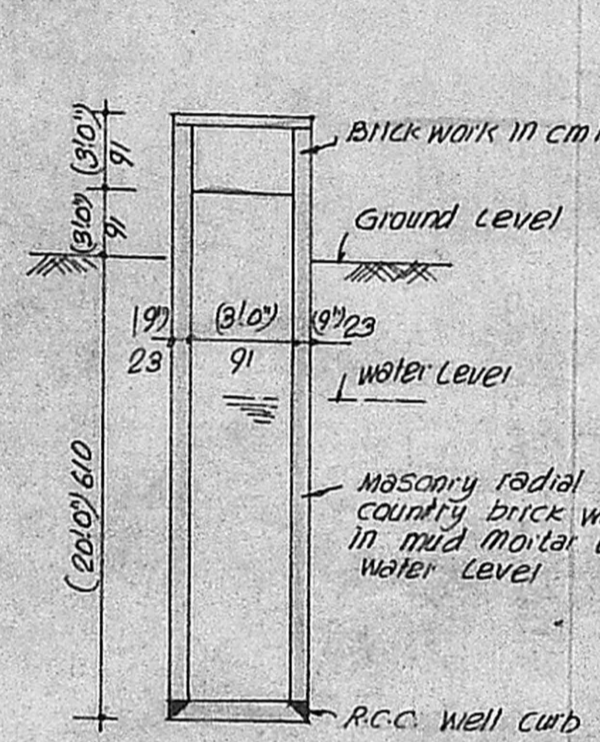
Section of 3.0" φ well
